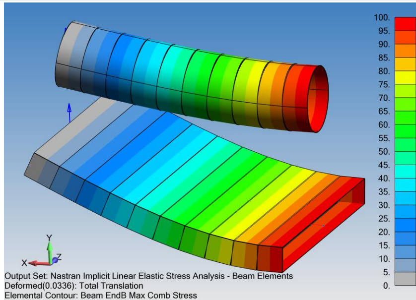
Nastran Results
