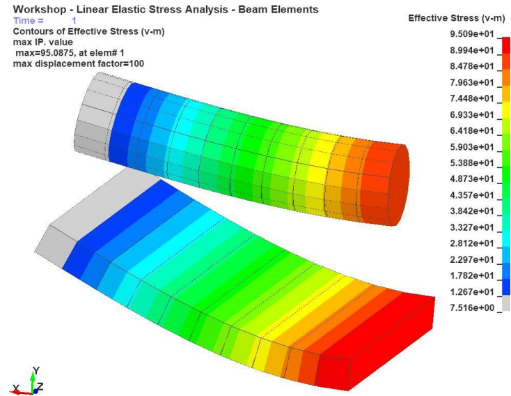
LS-DYNA Results
