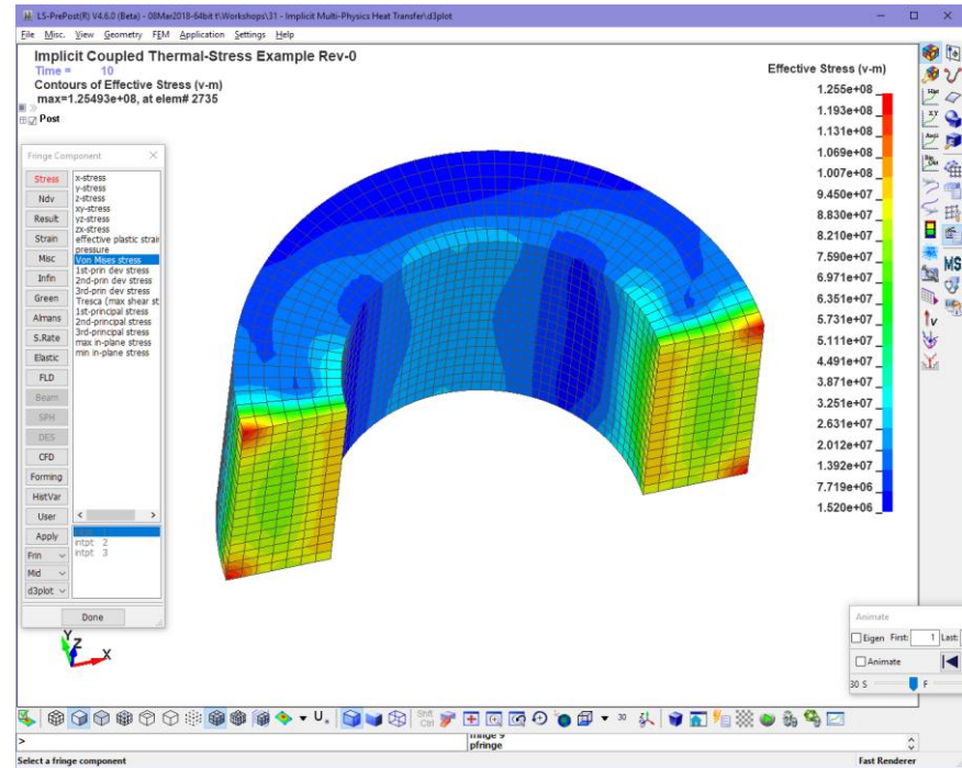
Stress Field (Fringe Component / Stress / Von Mises Stress)
