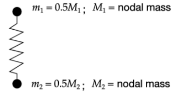
Figure 25.1. Lumped spring mass system.
